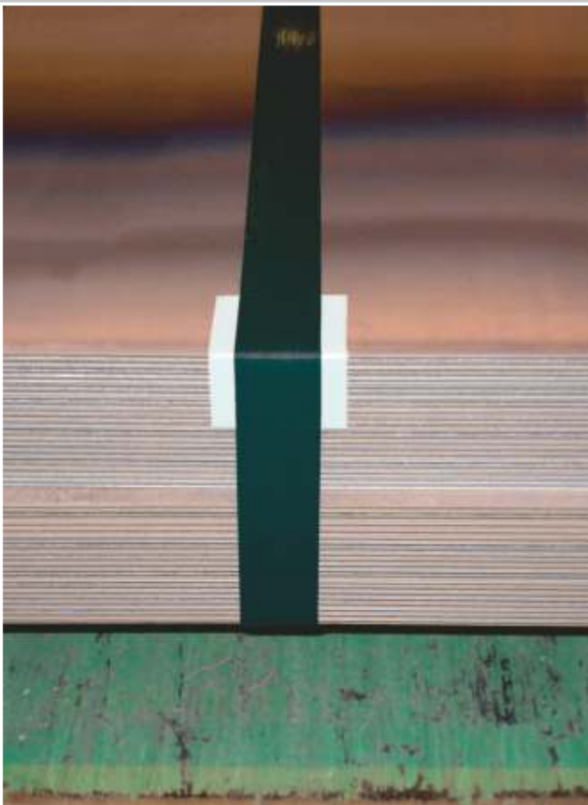
Common steel strapping with edge protection
